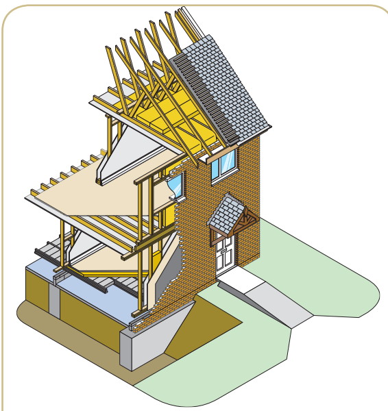
Typical timber frame construction
