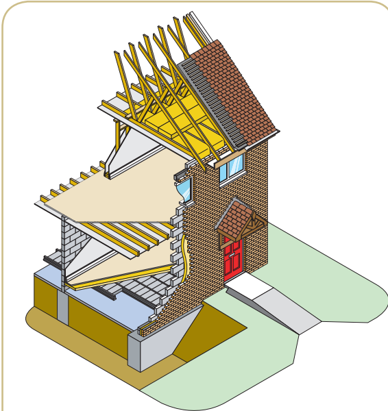
Typical masonry cavity construction
